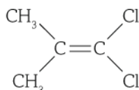
1, 1-dichloro-2,2-methylpropene
